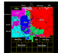
ARM1176JZ-S 1sq mm on 65nm (Metro™ libraries)
